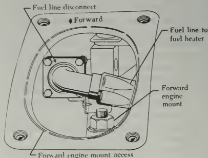
FIGURE 8-17. Fuel line disconnect.
